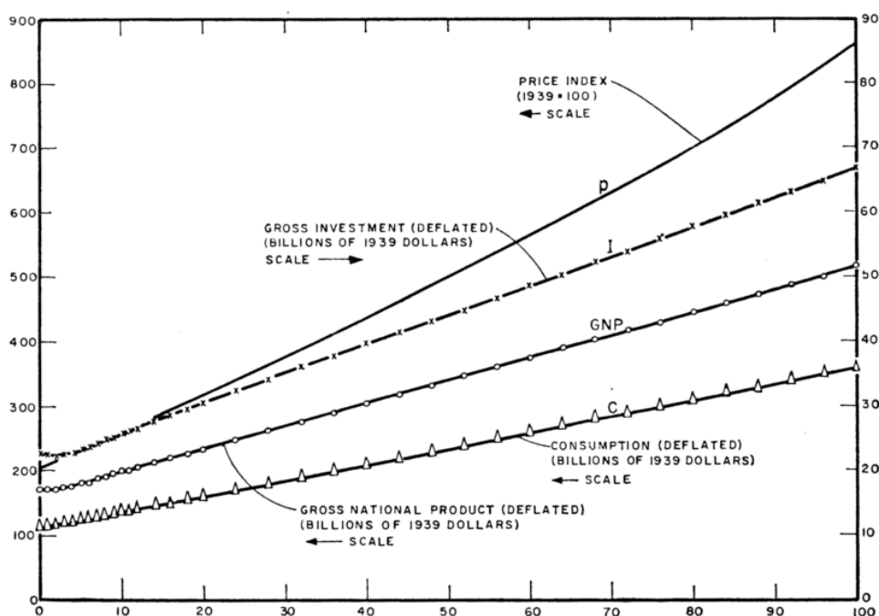
Figure 1: Klein-Goldberger Time Paths (without any shocks).
